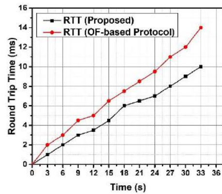
Fig. 9: Round-Trip Delay Comparison for 50 (Proposed) Nodes with respect to OF-based Protocol
