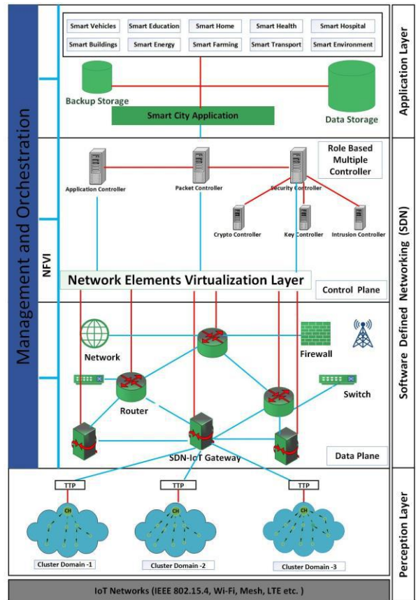
Fig. 4: Proposed “SDoT-NFV” Architecture.
