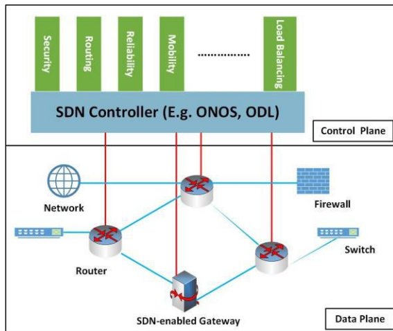
Fig. 1: SDN Architecture
