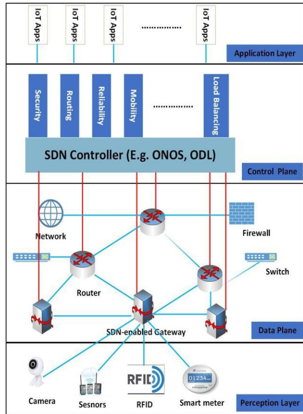
Fig. 2: SDN-IoT Architecture
