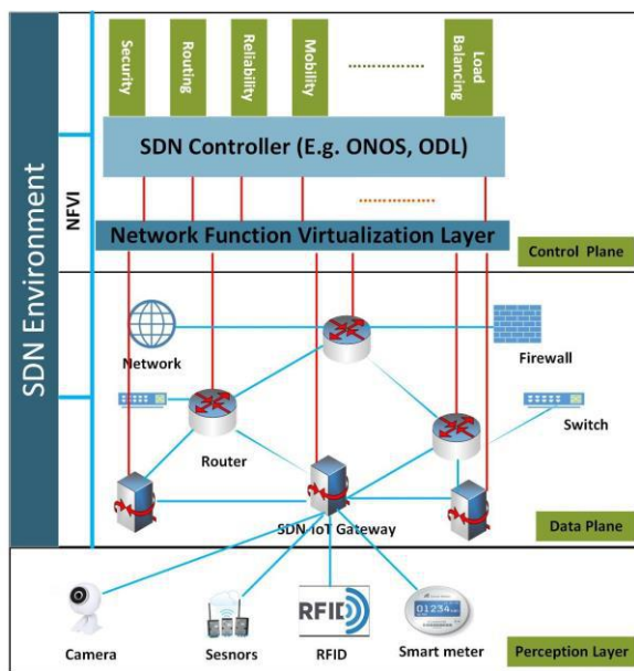
Fig. 3: NFV with SDN [29].
