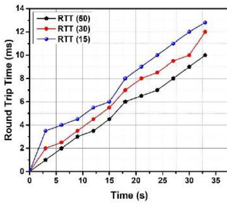
Fig. 8: Round-Trip Delay Comparison with respect to 15, 30 and 50 Nodes
